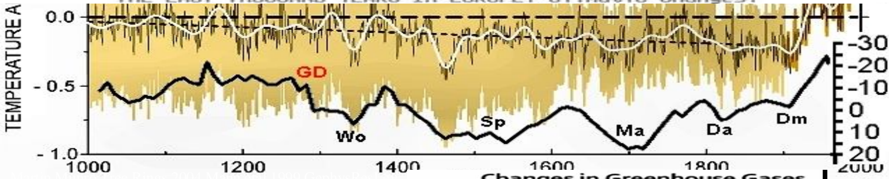
THE LAST THOUSAND YEARS IN EUROPE. Climatic changes.
