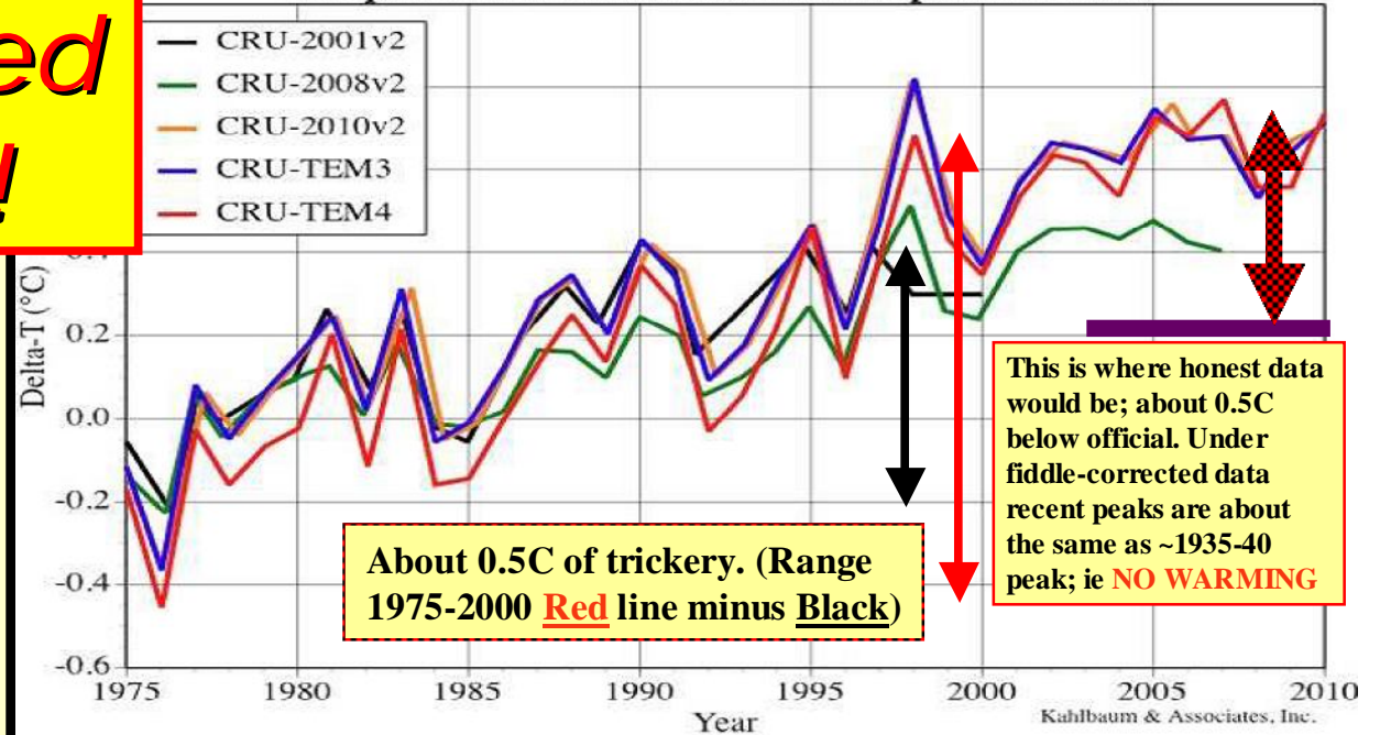
Comparison of CRU Global Annual Temperature Trends
