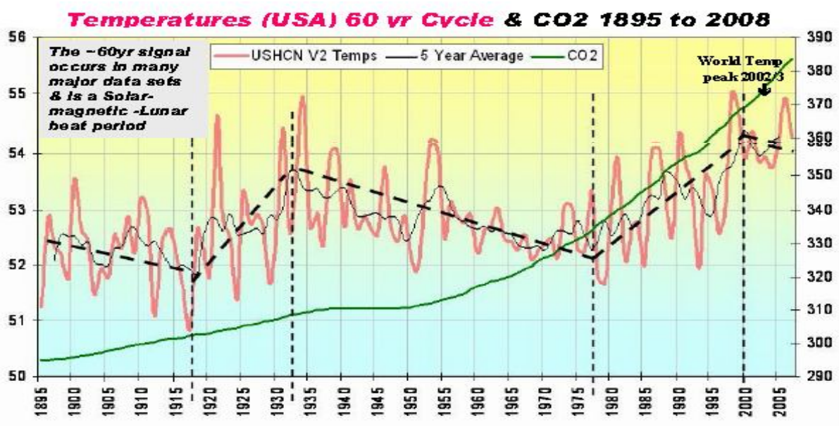
al data - Graph by JD'Aleo Sept 2008 Circulated by Piers Corbyn www.weatheraction.com
