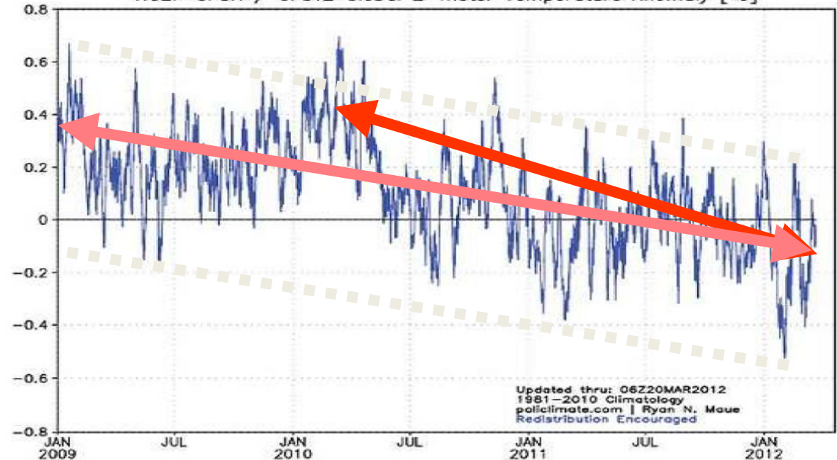
NCEP CFSR / CFSv2 Global 2-meter Temperature Anomaly [°C]
