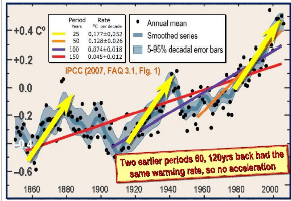
al data - Graph by JD'Aleo Sept 2008 Circulated by Piers Corbyn www.weatheraction.com
