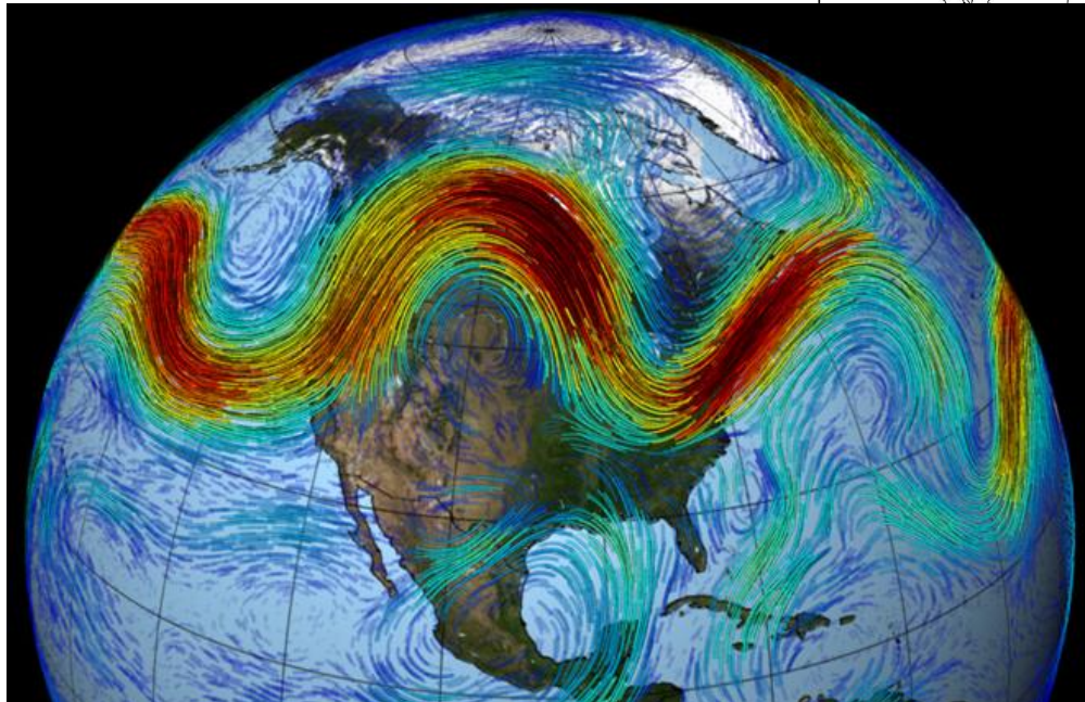
STATE UNIV | 1987-2016 HISTORICAL CLIMATOLOGY
